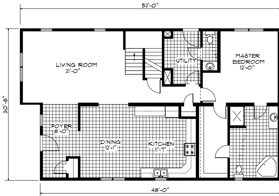
FIRST FLOOR 1,533 SQ. FT.
