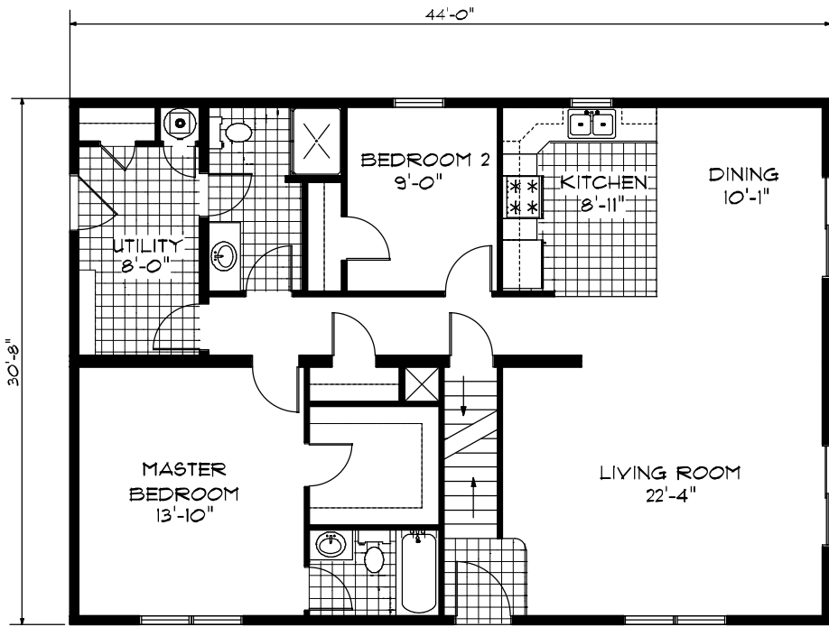
FIRST STORY 1,349 SQ. FT.
