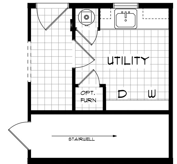
STAIRWELL OPTION
